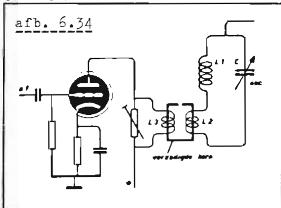
schematisch, de Saturated core modulation.
